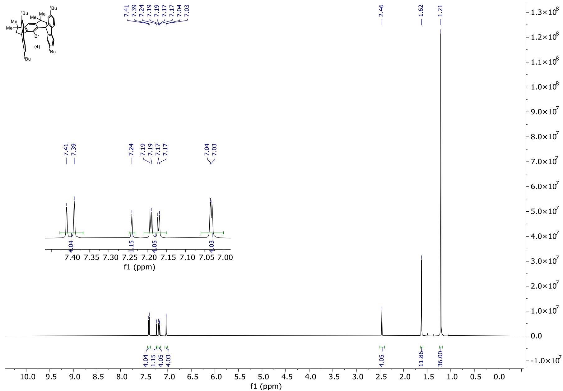
^1\text{H} NMR of ^t\text{Bu} -MsFluidBr ( 4 ) (400 MHz, \text{CDCl}_3 )
